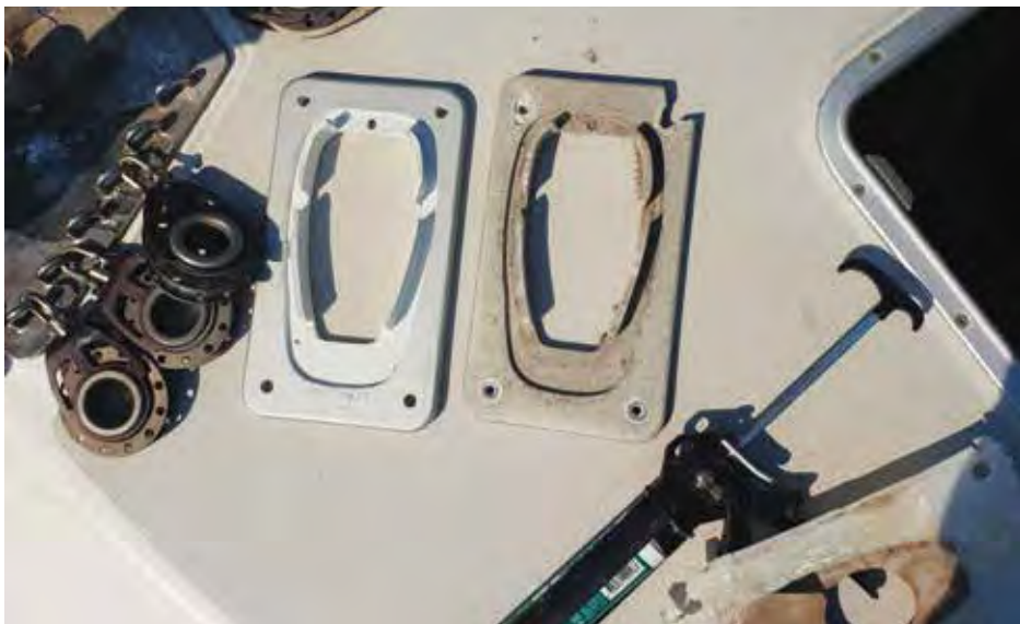
Old vs new—look closely and you can see the corrosion in both the aft bolt holes.
